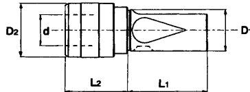
Rigid Tap Holders Straight Shank
