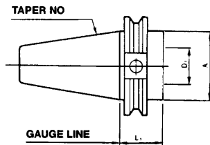
CT Shanks
