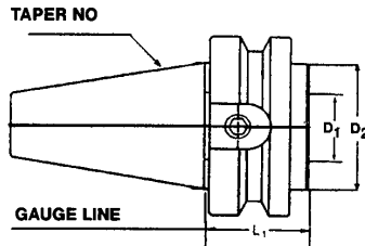
BT Shanks
