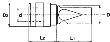
Rigid Tap Holders Straight Shank
